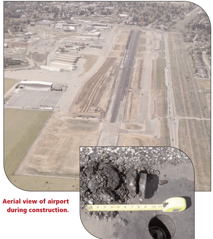
Typical core shows deteriorated asphalt.
